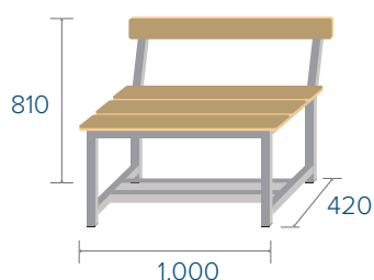
BANC-4-1000 11,5kg · 0,34m 3
