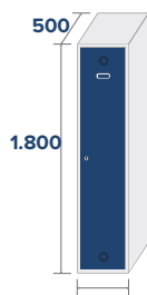
ECO-40/1 COD:84001 20,3kg,0,36m 3
