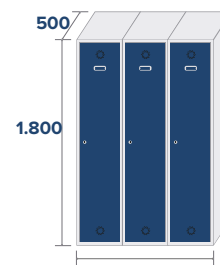
ECO-40/3 COD:84003 49,9kg,1,08m 3
