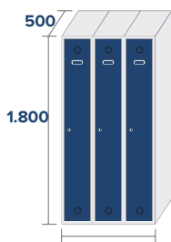
ECO-30/3 COD:83003 46kg,0,81m 3
