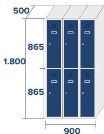
ECO-30/3 COD: 83013 47,3kg,0,81m 3
