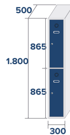
ECO-30/1 COD: 83011 19,1kg,0,27m 3
