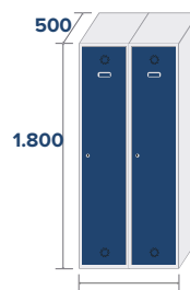
ECO-40/2 COD:84002 35,1kg,0,72m 3
