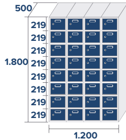
ECO-30/4 COD: 83824 91,8kg, 1,08m 3
