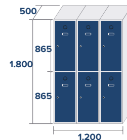
ECO-40/3 COD: 84013 59kg,1,08m 3
