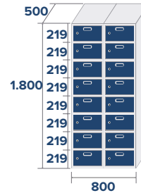
ECO-40/2 COD: 84822 56,8kg, 0,72m 3
