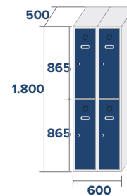
ECO-30/2 COD: 83012 33,2kg,0,54m 3
