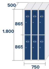
ECO-25/3 COD: 82513 44,2kg,0,67m 3
