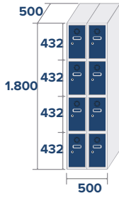
ECO-25/2 COD: 82522 35,6kg 0,45m 3
