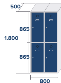
ECO-40/2 COD: 84012 41kg,0,72m 3
