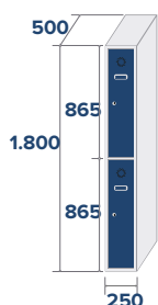
ECO-25/1 COD: 82511 18,4kg,0,22m 3
