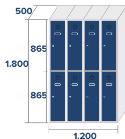
ECO-30/4 COD: 83014 61,4kg,1,08m 3
