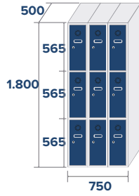
ECO-25/3 COD: 82533 47,7kg 0,67m 3
