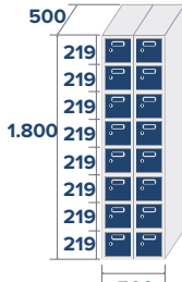
ECO-25/2 COD: 82582 43,8kg, 0,45m 3
