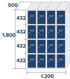
ECO-30/4 COD: 83024 71,2kg 1,08m 3
