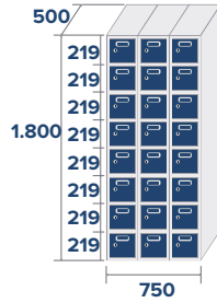
ECO-25/3 COD: 82583 63,2kg, 0,67m 3
